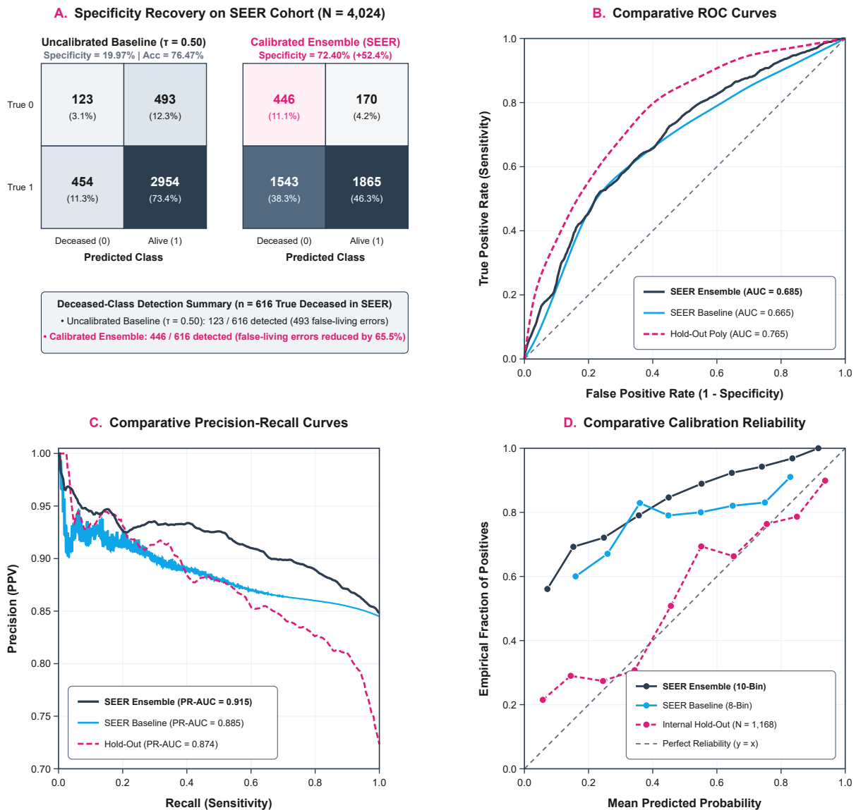
Figure 2. Comparative External Validation Diagnostics on the Independent SEER Cohort ( N = 4024 )
