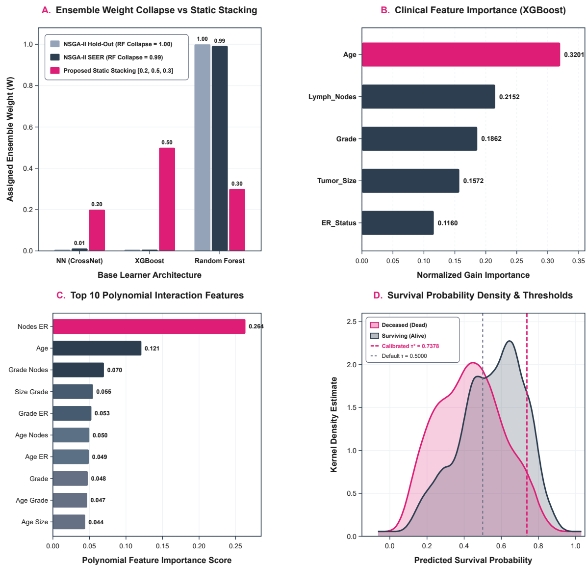
Figure 3. Ensemble Weight Mechanics, Clinical Feature Importance, Polynomial Interactions, and Risk Stratification
