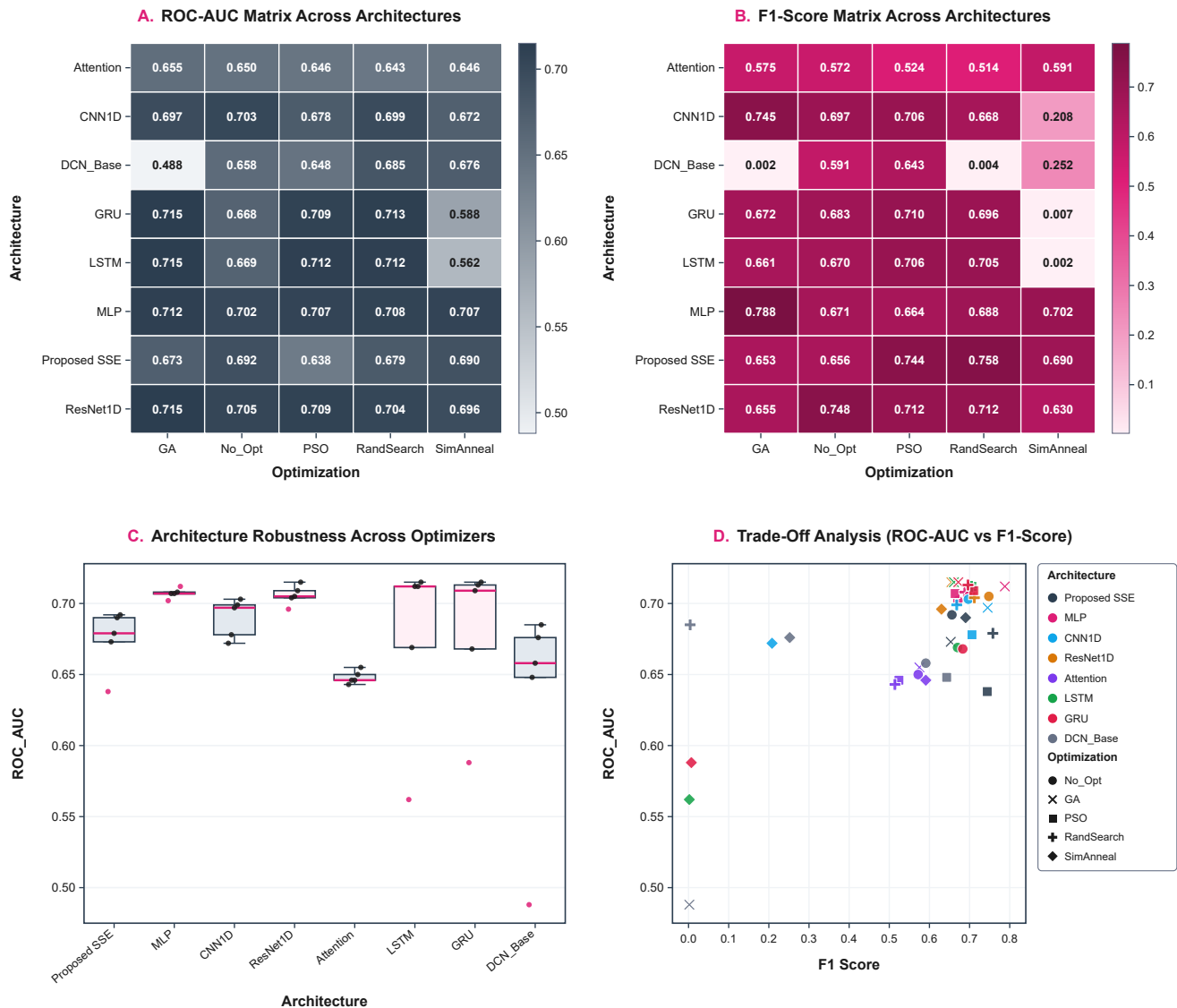
Figure 4. Comprehensive Architecture and Optimizer Benchmark Summary Across 40 Configurations on SEER ( N = 4024 )
